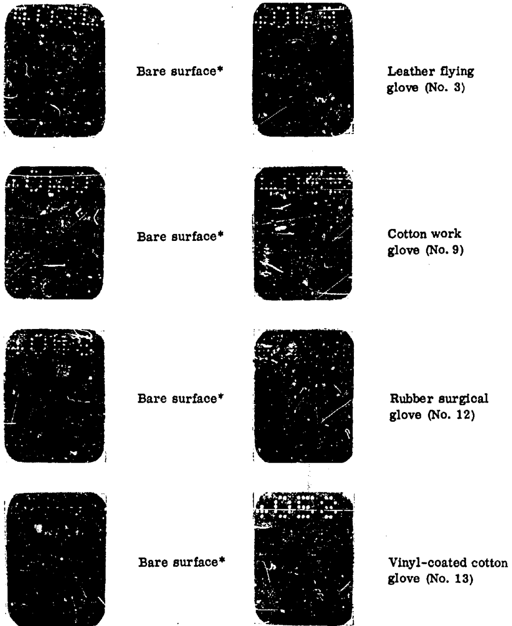
Figure 3.5 Radioautographs of leading edge of the wing of a B-57B with and without interposition of glove swatches.
